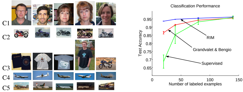
Figure 4: Left: Randomly chosen example images from clusters discovered by unsupervised RIM on Caltech Image. Right: Semi-supervised learning on Caltech Images.
